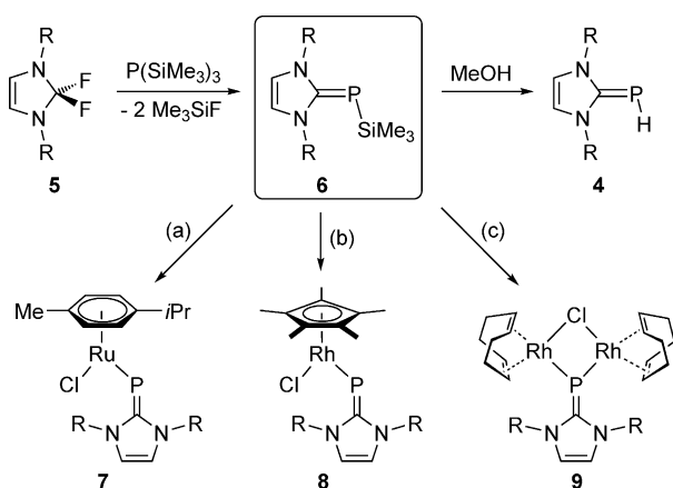
Scheme 1. Synthesis of carbene–phosphinidyne transition metal complexes; R = 2,6-diisopropylphenyl (Dipp); a) 0.5 equiv [(\eta^6\text{-}p\text{-cymene})\text{RuCl}_2]_2 , b) 0.5 equiv [(\eta^5\text{-C}_5\text{Me}_5)\text{RhCl}_2]_2 , c) 1.0 equiv [\text{Rh}(\text{cod})\text{Cl}]_2 .
