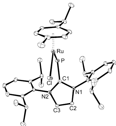
Figure 4. ORTEP diagram of 7 with thermal displacement parameters drawn at 50% probability level. Selected bond length [Å] and angles [°]: Ru–P 2.2099(6), Ru–Cl 2.3956(6), P–C1 1.824(2), N1–C1 1.363(3), N2–C1 1.360(3); Ru–P–C1 112.80(7), P–Ru–Cl 94.24(2), P–C1–N1 123.67(16), P–C1–N2 129.41(17), N1–C1–N2 105.47(18).
